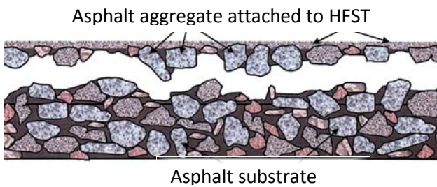
FIGURE 21 – Shallow tearing.
